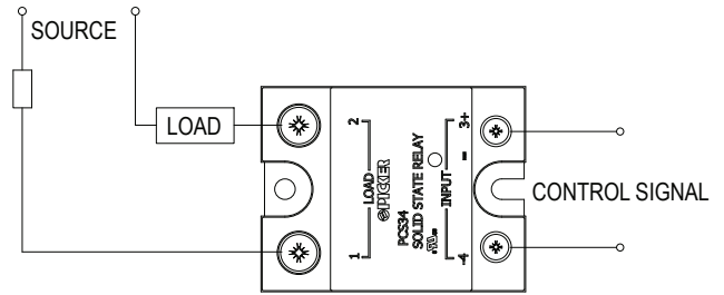
Wiring Diagram
